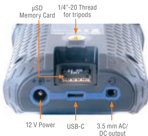
Meter Ports
